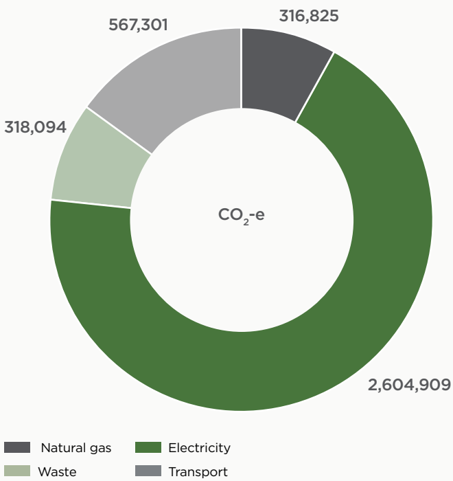
Figure 55: Emission sources 2020
